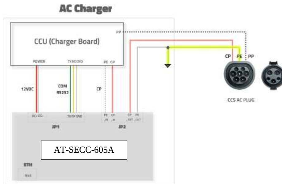
Figure 4: Wiring with External AC Charger Board/Controller
