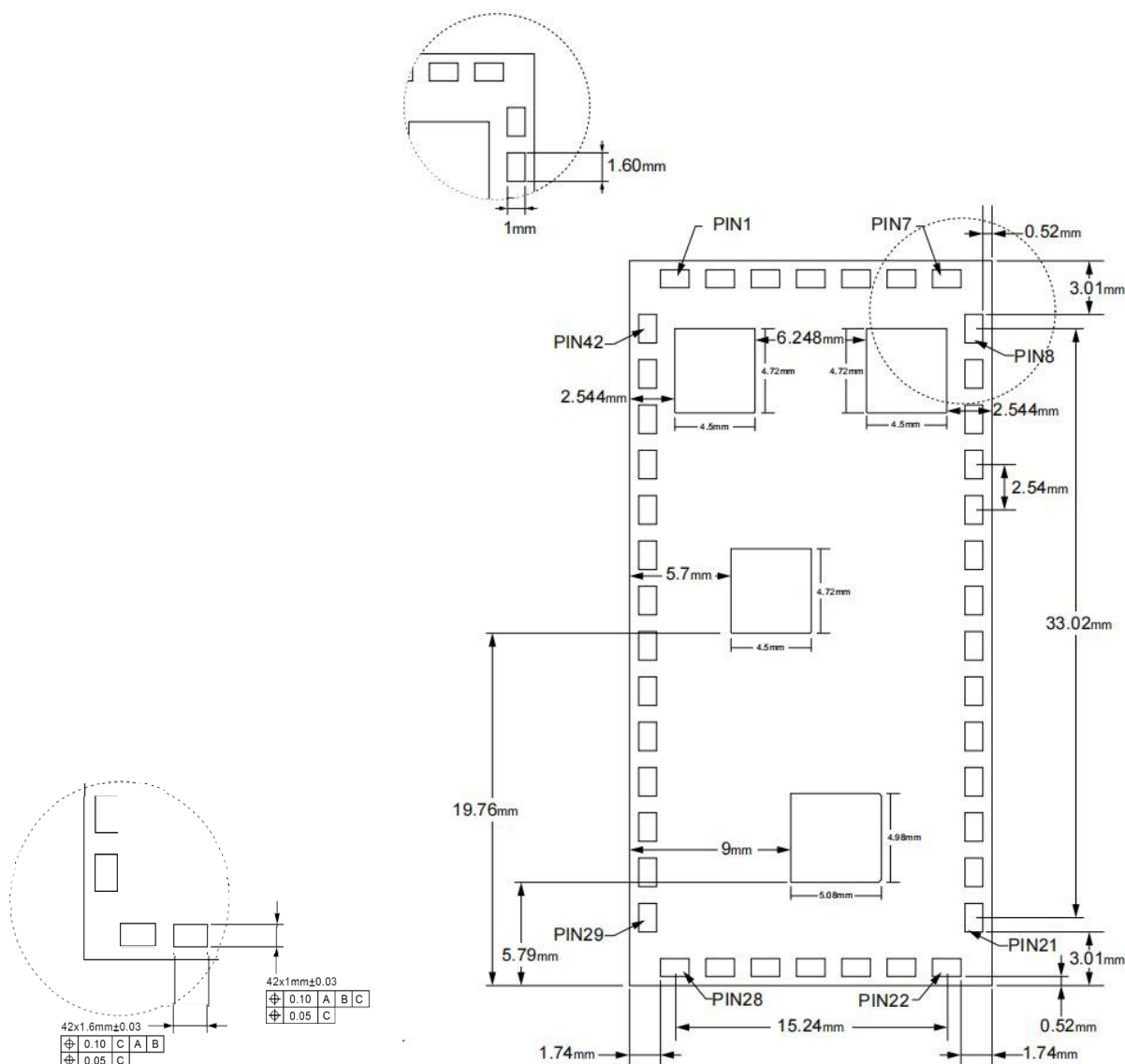
Figure 5 – Recommended Footprint
