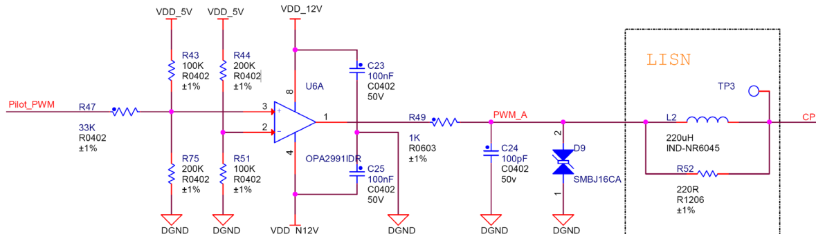
Figure 10 – Control Pilot Signal Generation
