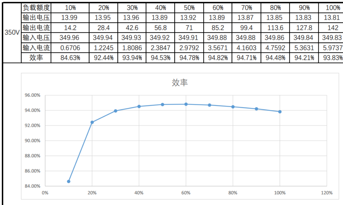
DC efficiency curve
