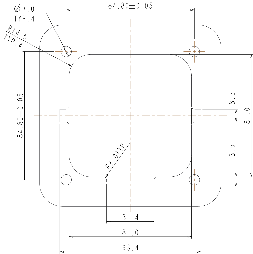
REAR MOUNTED FLANGE 后安装法兰尺寸
