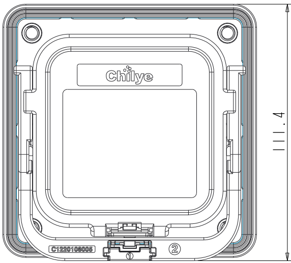
AFTER MATING 2-M8X1.25 配合锁紧状态 LENGTH 15MM
