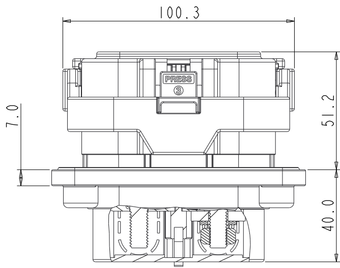
AFTER MATING 2-M8X1.25 配合锁紧状态 LENGTH 15MM
