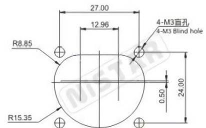
安装开孔尺寸 Install the panel opening Size
